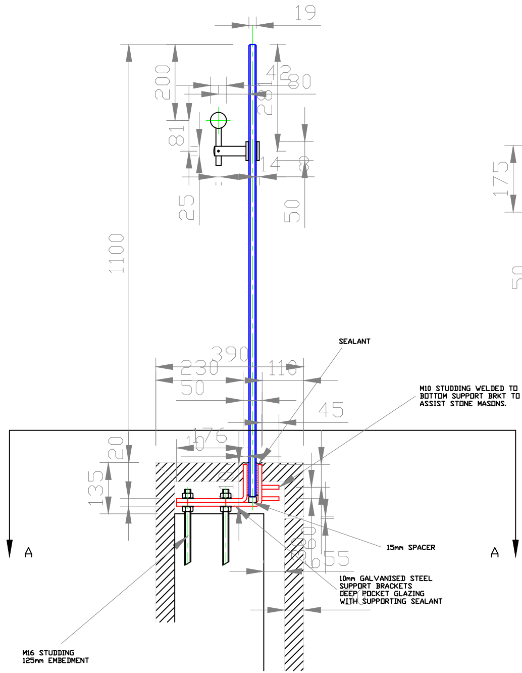
SIDE ELEVATION SCALE 1/5 TYPICAL FIXING ARRANGEMENT
